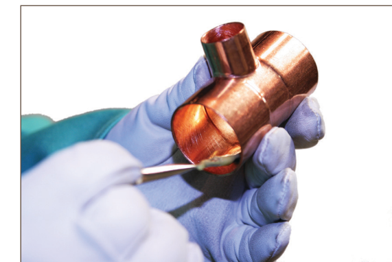
Figure 7.10. Fluxing: Fitting
