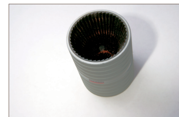
Figure 11.9. Combination tool for I.D and burr removal
