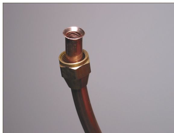
Figure 9.5. Completed Flared Tube End
