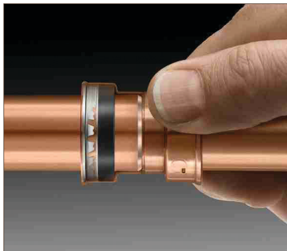
Figure 12.12. Completed installation of a push-connect joint
