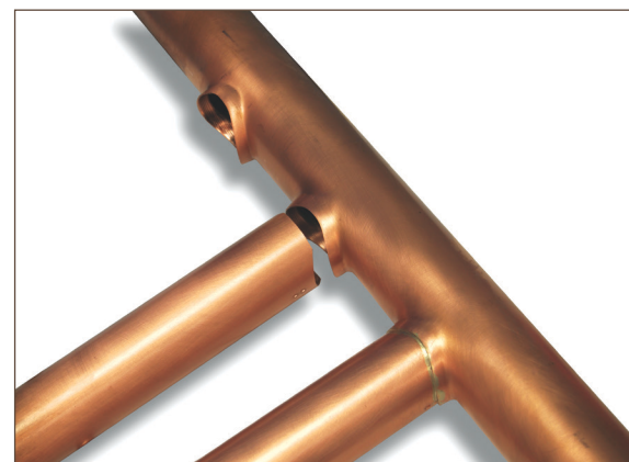
Figure 13.1. Mechanically formed extruded outlet requires only one brazed joint
