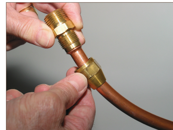
Figure 9.1. Flare Fitting/Flared Joint During Assembly
