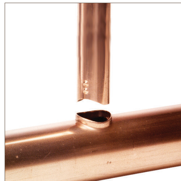
Figure 13.11. Aligning the dimples with the run of the tube
