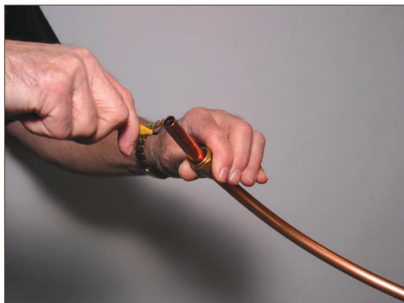
Figure 9.3. Reaming Prior to Flaring the Tube End
