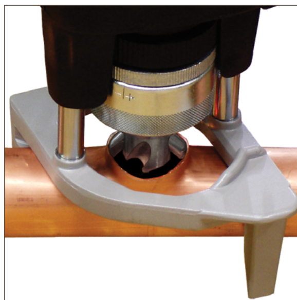
Figure 13.7. Forming the outlet
