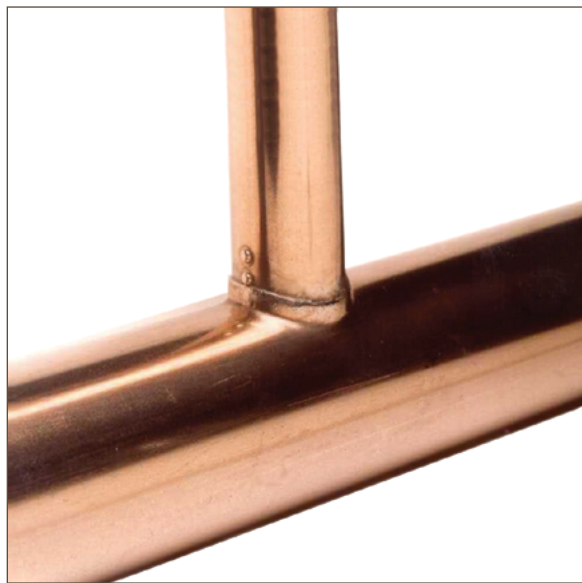
Figure 13.12. Finished joint
