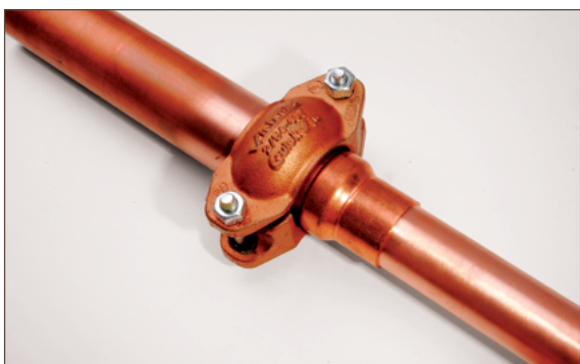
Figure 10.10. Assembled joint
