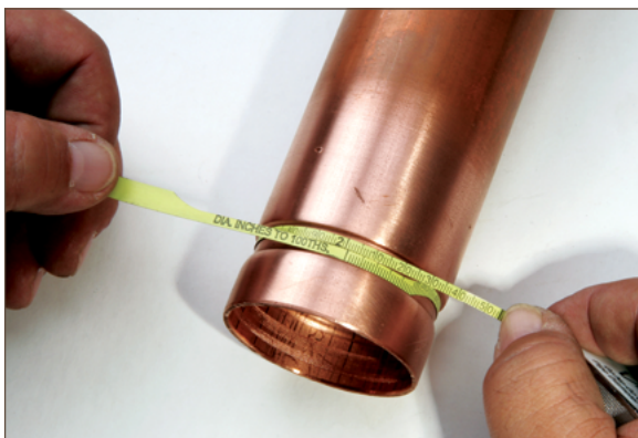
Figure 10.5. Grooved tube end
